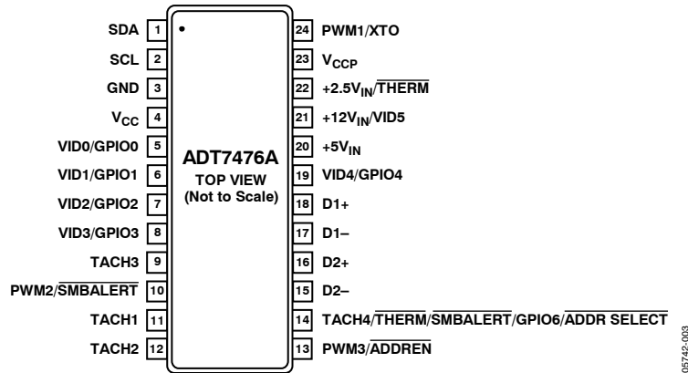
Figure 3. Pin Configuration
