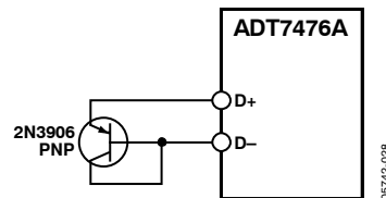
Figure 27. Measuring Temperature Using a PNP Transistor
