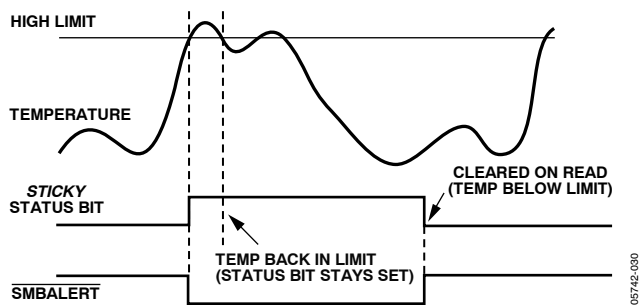
Figure 29. \overline{\text{SMBALERT}} and Status Bit Behavior
