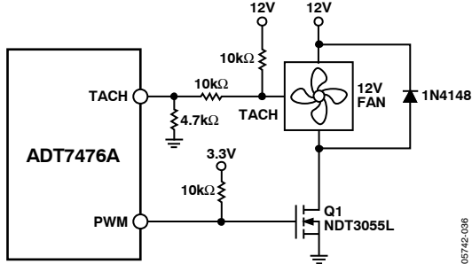
Figure 35. Driving a 3-Wire Fan Using an N-Channel MOSFET
