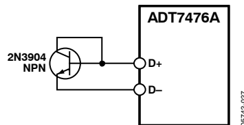
Figure 26. Measuring Temperature Using an NPN Transistor
